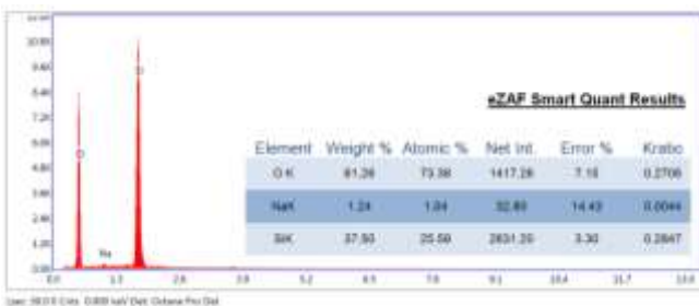
Figure 10. elemental analysis of reclaimed silica sand after third washing by EDS spectrometer
